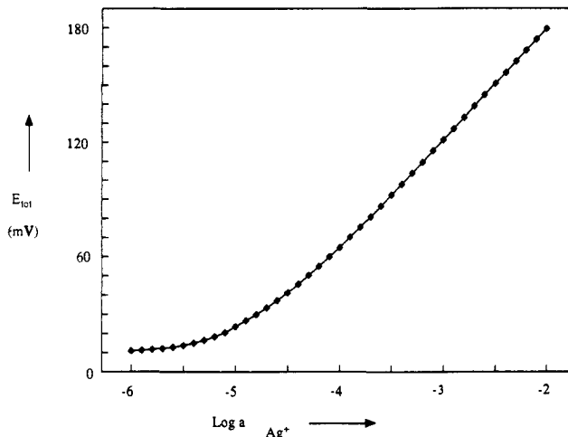
Figure 2. Ag + responses of CHEMFETs containing calix[4]arene ionophore 2 in the presence of 0.1 M Ca(NO 3 ) 2 .
