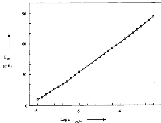
Figure 6. Pb 2+ response of CHEMFETs containing calix[4]arene ionophore 29 in the presence of 1 M KCl.
